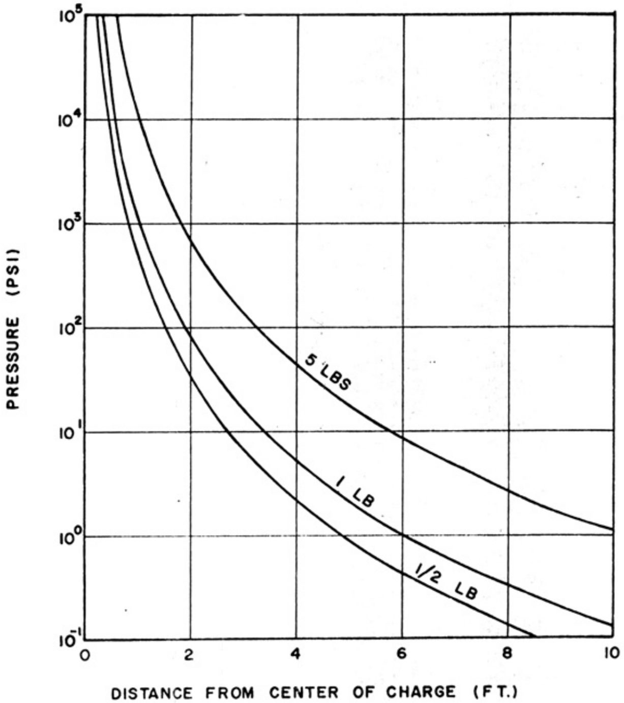
Fig. III-C-1. An Approximate Pressure-Distance Relationship For the Detonation Products of a Spherical Charge Detonated in a Vacuum
